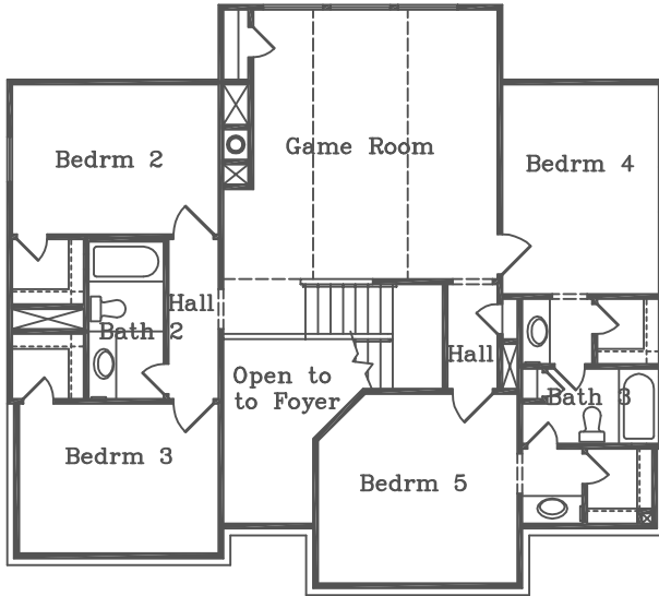
2ND FLOOR
